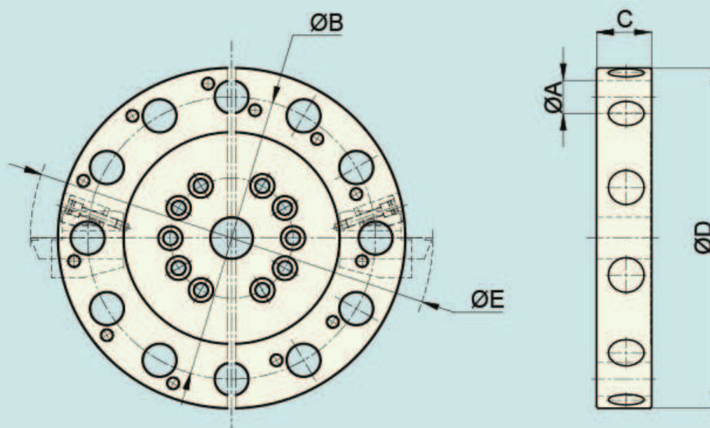
VDI Tool Disc for 12 Stations
